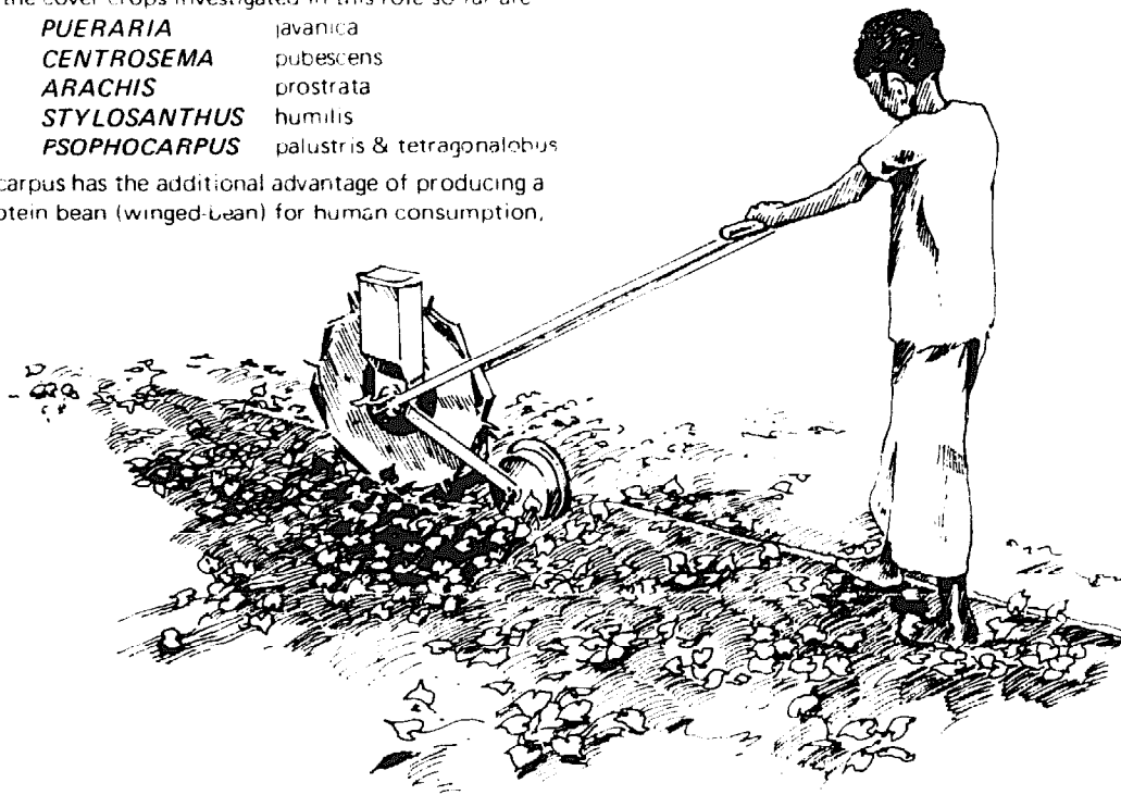
Injection planting through live mulch
